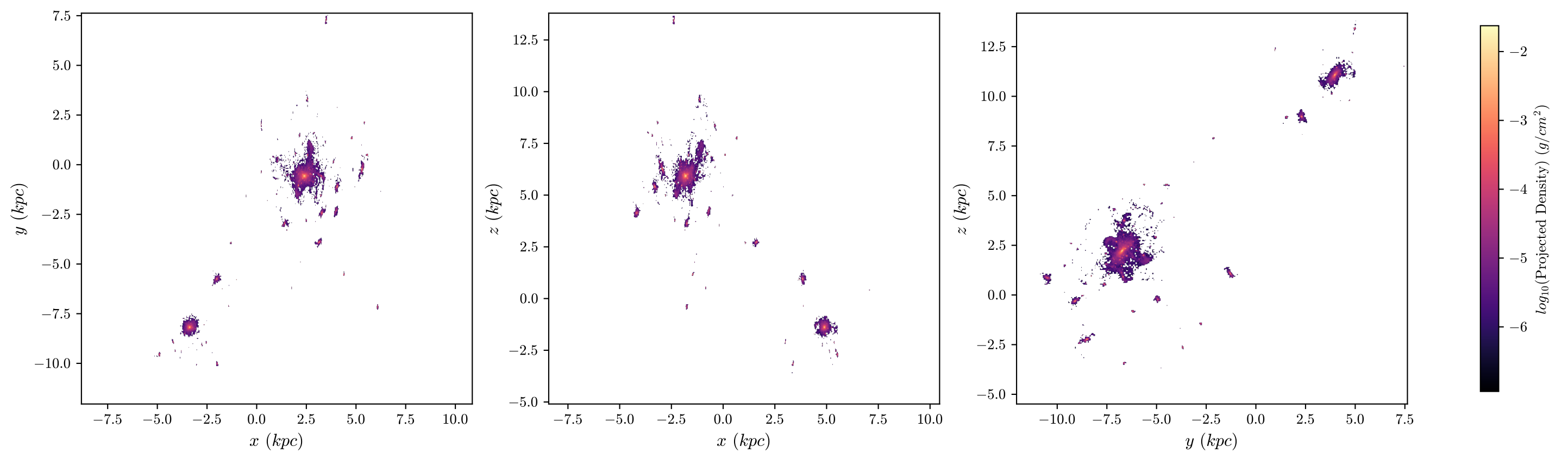
halo8 Stars, z = 3.263 , 512 bins
