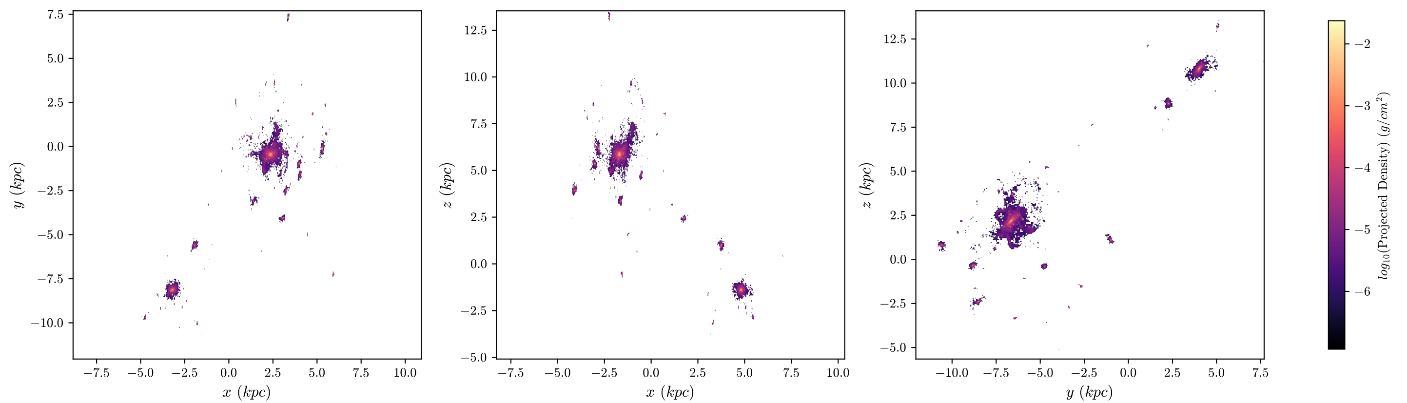
halo8 Stars, z = 3.243 , 512 bins
