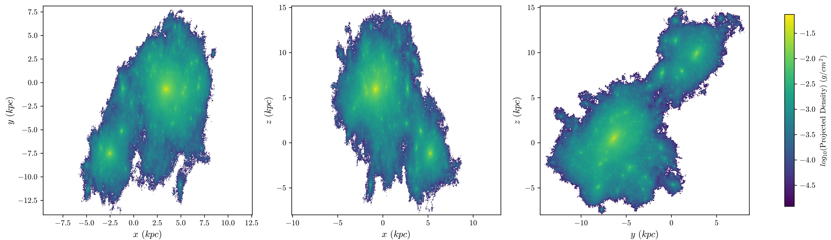
halo8 Stars, z = 3.203 , 512 bins
