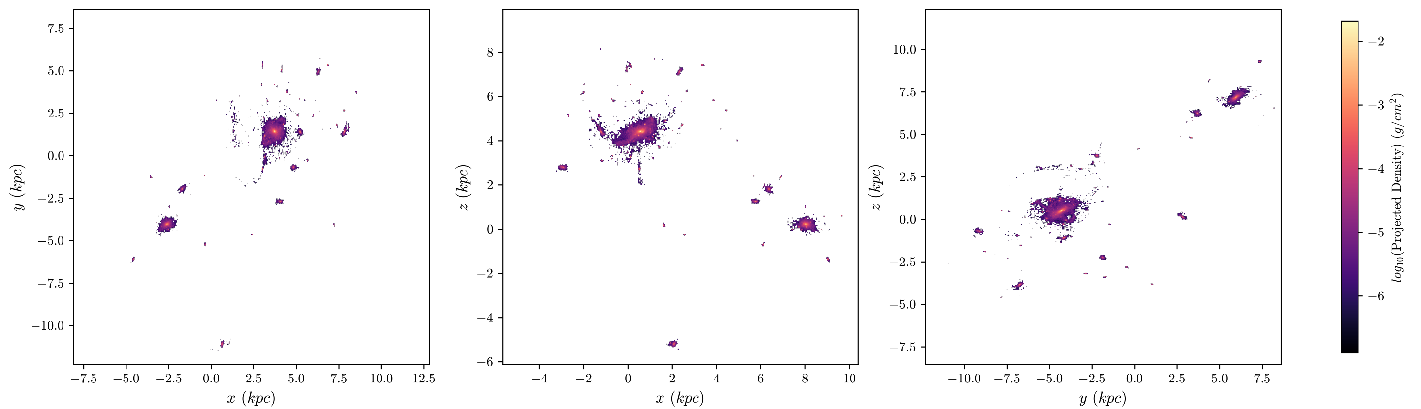
halo8 Stars, z = 3.085 , 512 bins
