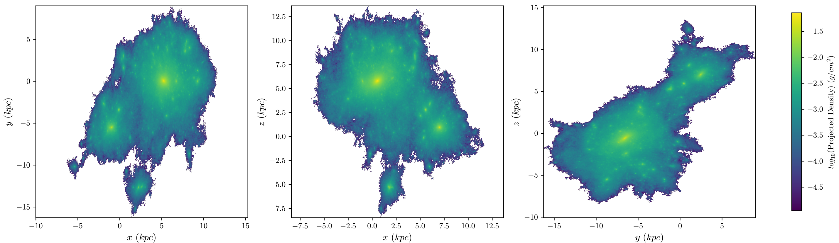
halo8 Stars, z = 3.085 , 512 bins
