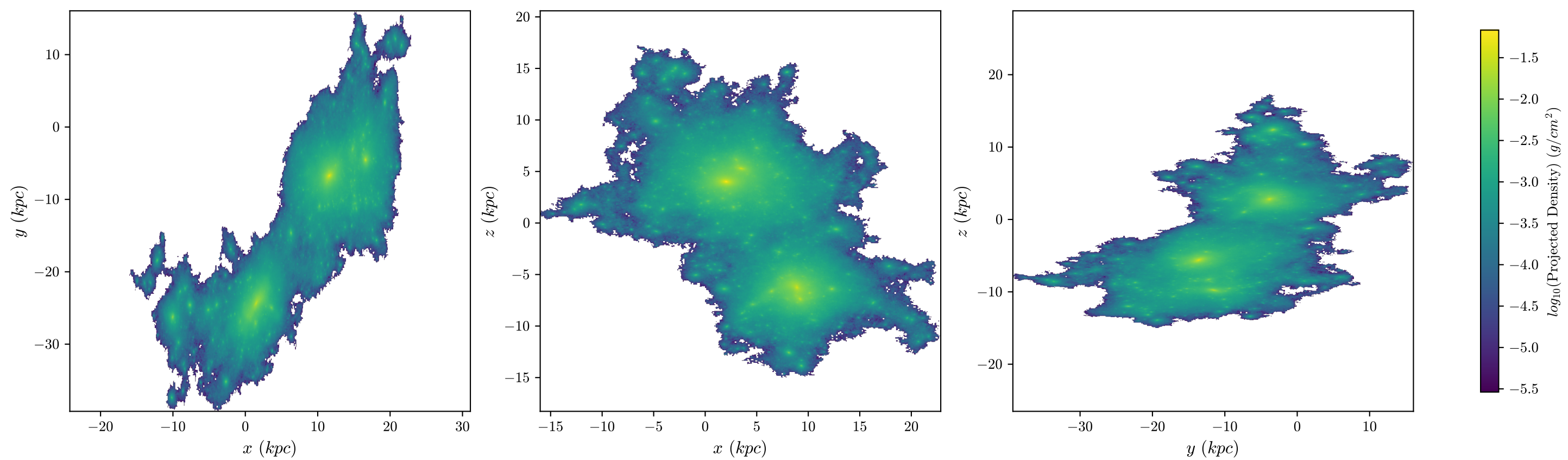
halo8 Stars, z = 2.178 , 512 bins
