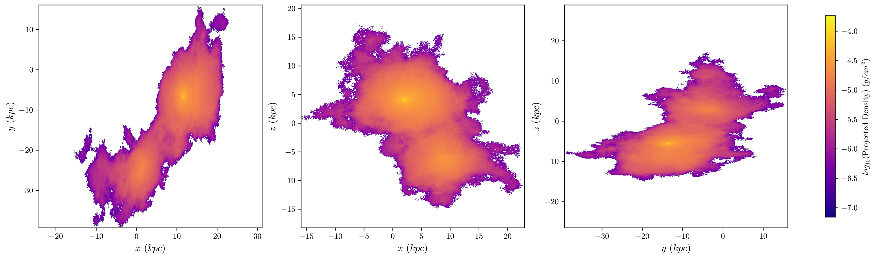
halo8 Dark Matter, z = 2.178 , 512 bins
