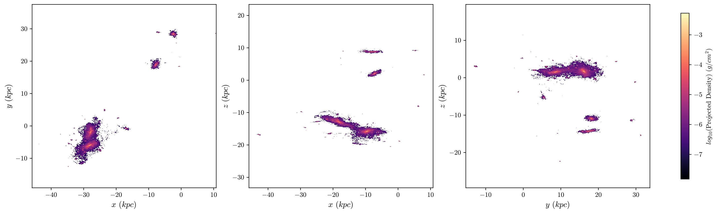
halo8 Stars, z = 1.496 , 512 bins
