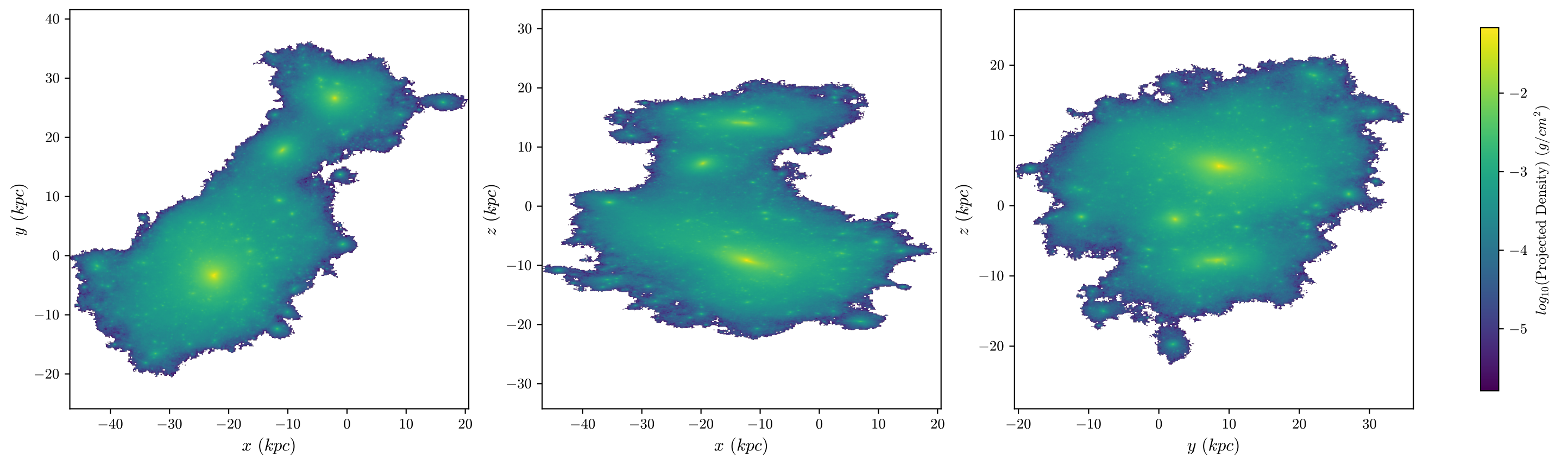
halo8 Stars, z = 1.324 , 512 bins
