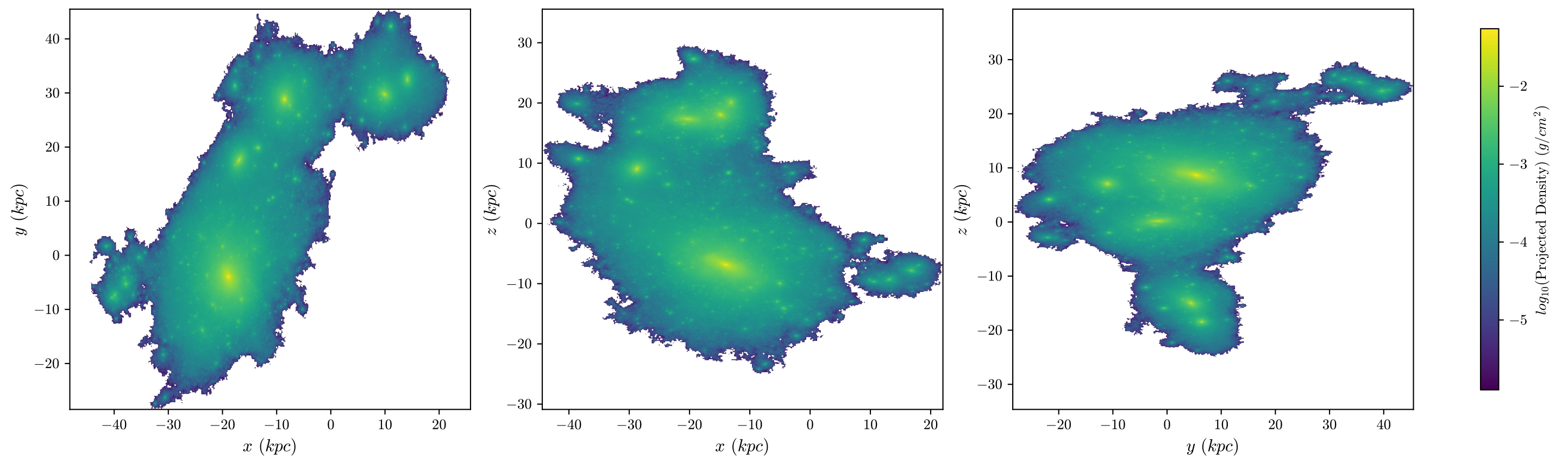
halo8 Stars, z = 1.185 , 512 bins
