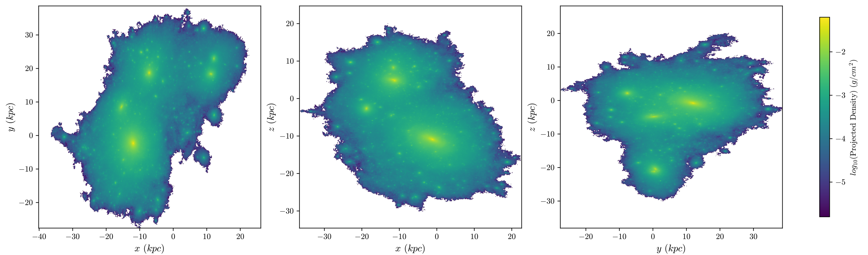
halo8 Stars, z = 1.065 , 512 bins
