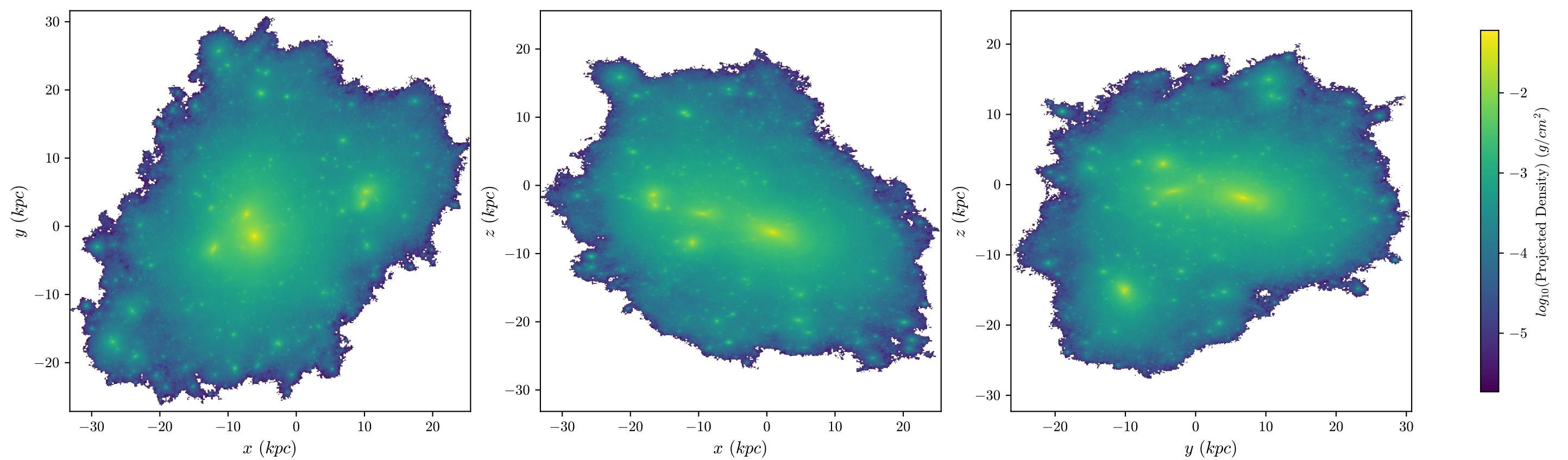
halo8 Stars, z = 0.96 , 512 bins
