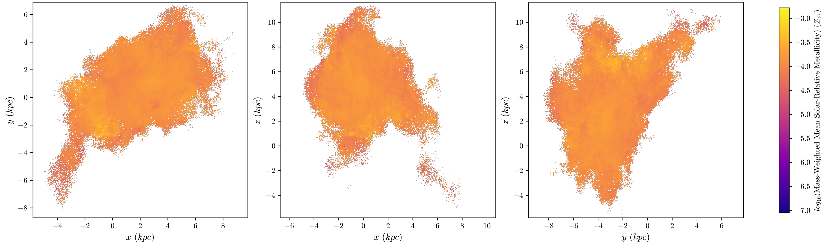
halo8 Mass-Weighted Mean Metallicity, z = 3.984 , 512 bins
