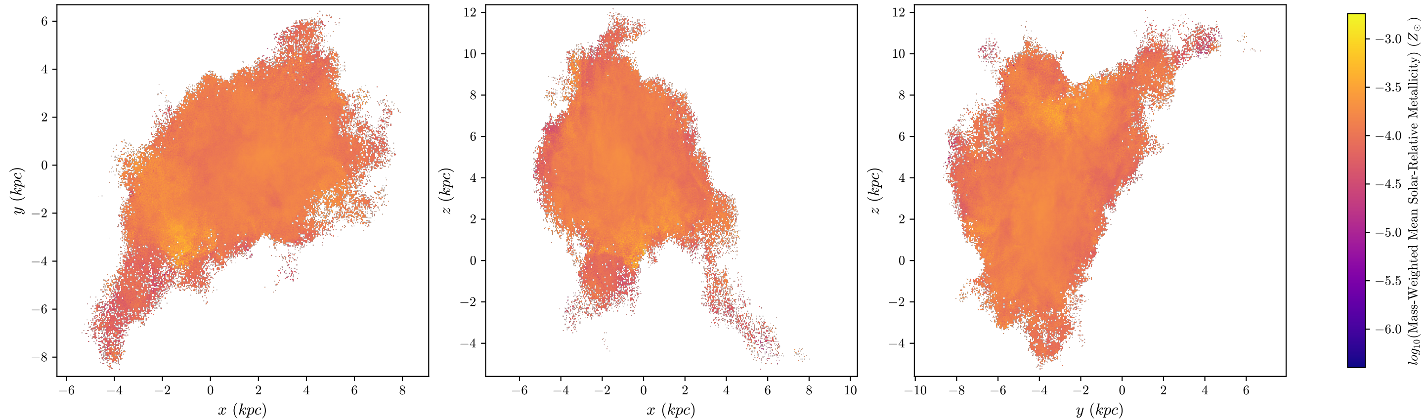
halo8 Mass-Weighted Mean Metallicity, z = 3.914 , 512 bins
