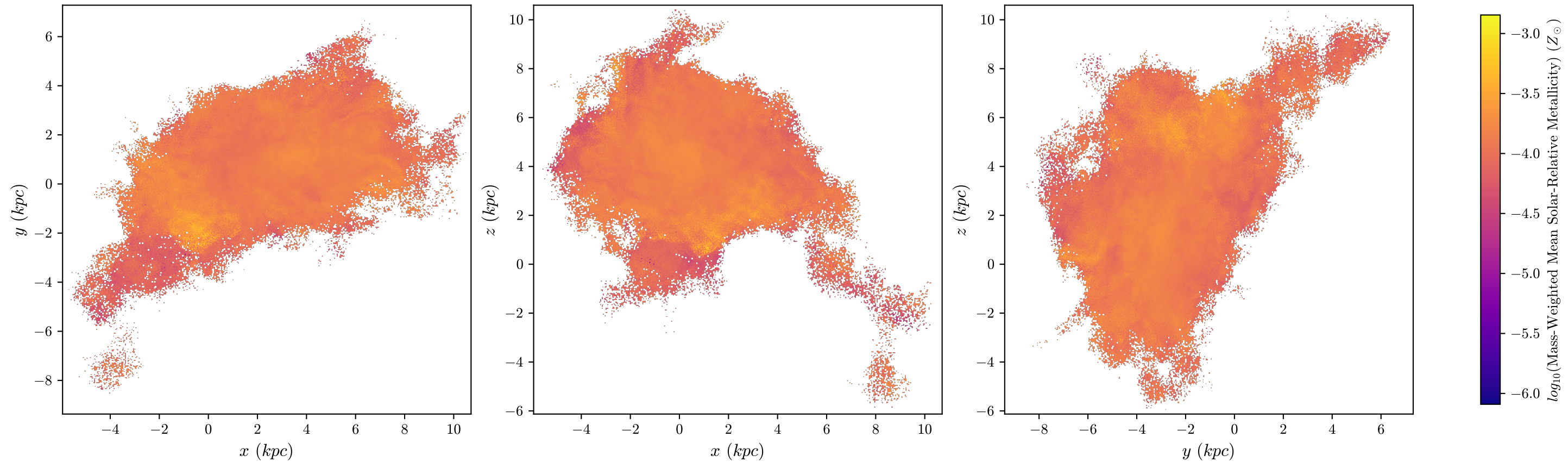
halo8 Mass-Weighted Mean Metallicity, z = 3.868 , 512 bins
