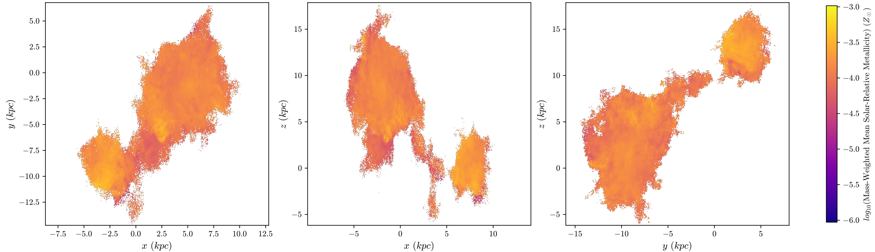
halo8 Mass-Weighted Mean Metallicity, z = 3.822 , 512 bins
