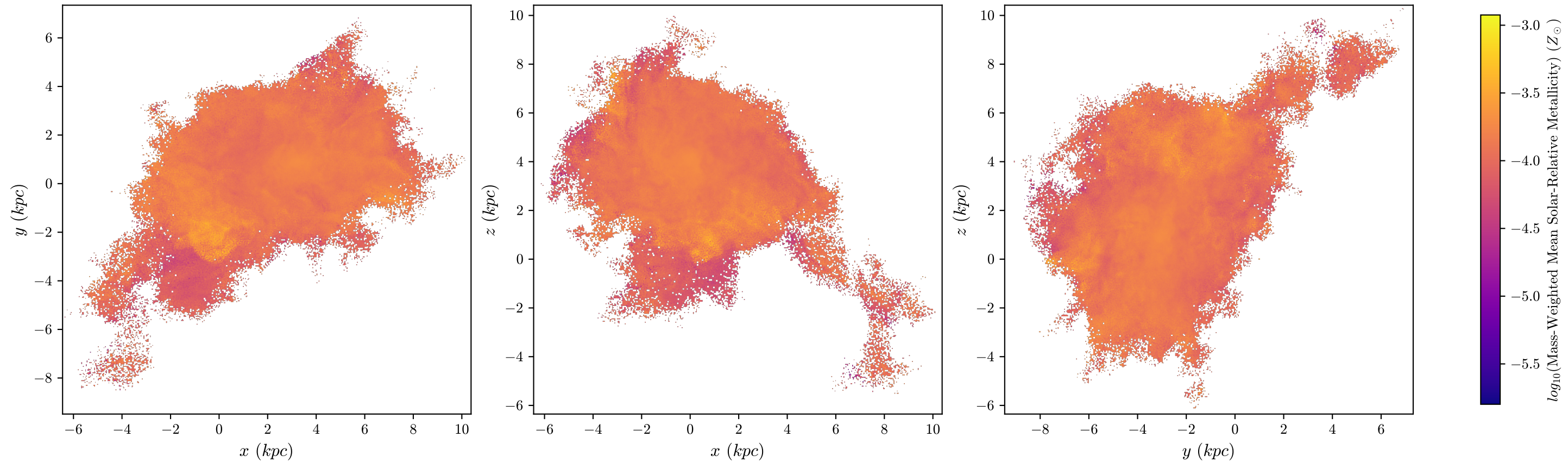
halo8 Mass-Weighted Mean Metallicity, z = 3.776 , 512 bins
