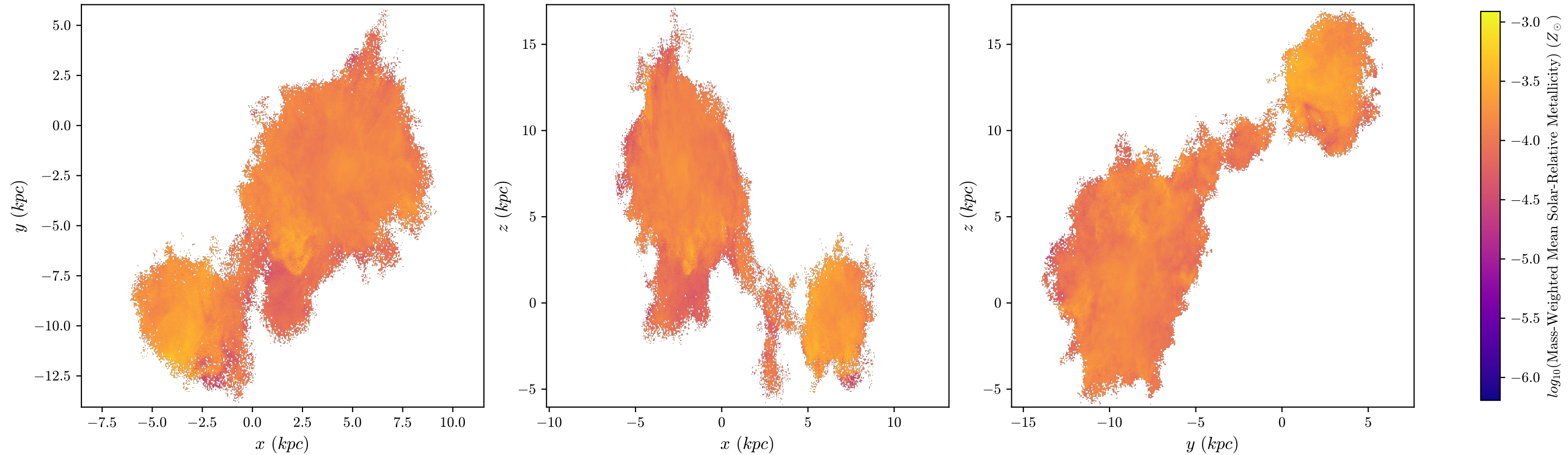
halo8 Mass-Weighted Mean Metallicity, z = 3.731 , 512 bins
