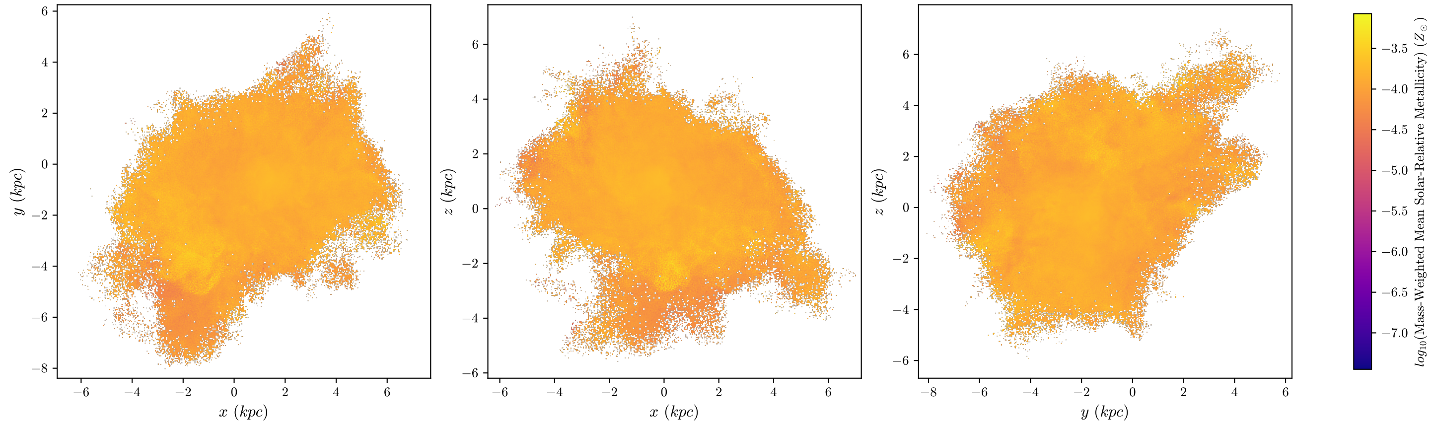
halo8 Mass-Weighted Mean Metallicity, z = 3.687 , 512 bins
