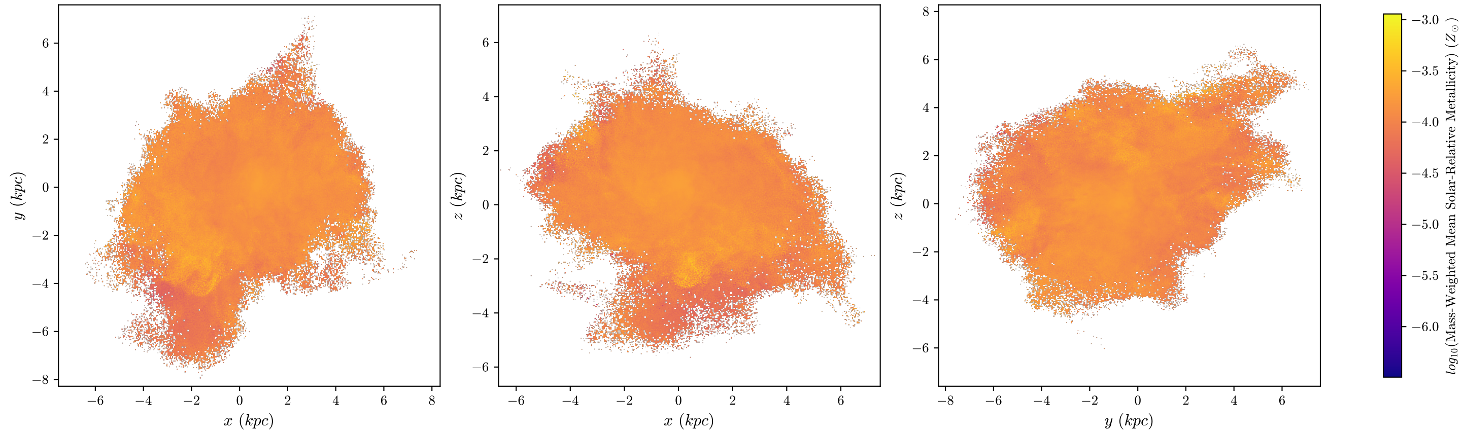
halo8 Mass-Weighted Mean Metallicity, z = 3.642 , 512 bins
