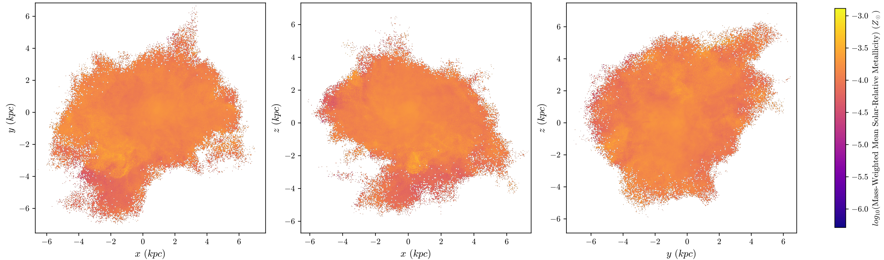
halo8 Mass-Weighted Mean Metallicity, z=3.62 , 512 bins
