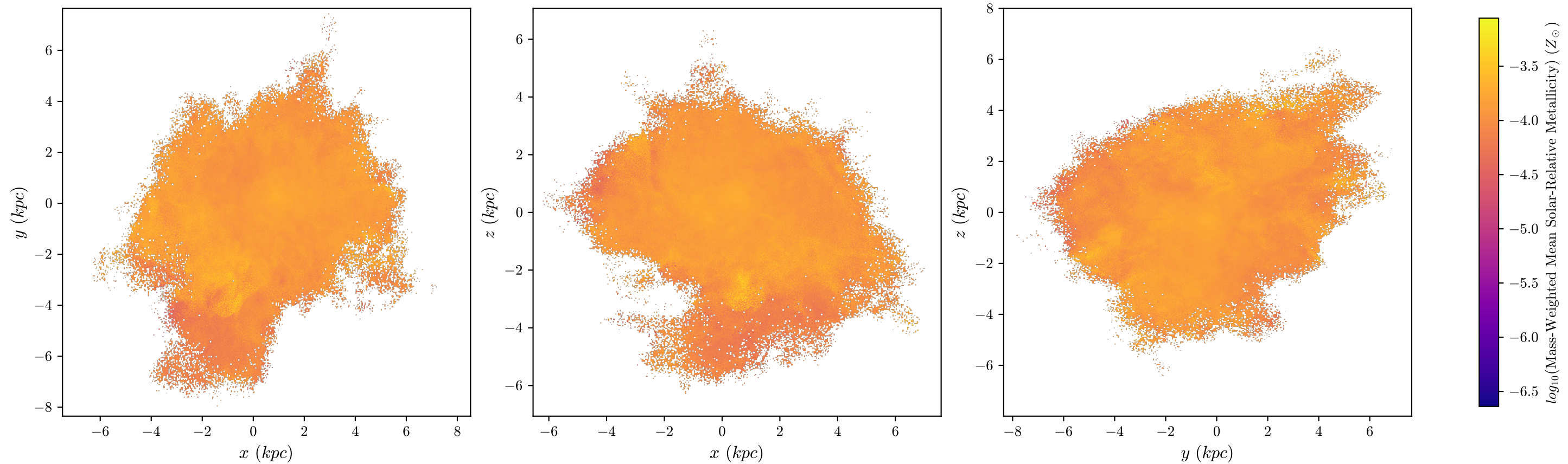
halo8 Mass-Weighted Mean Metallicity, z = 3.577 , 512 bins
