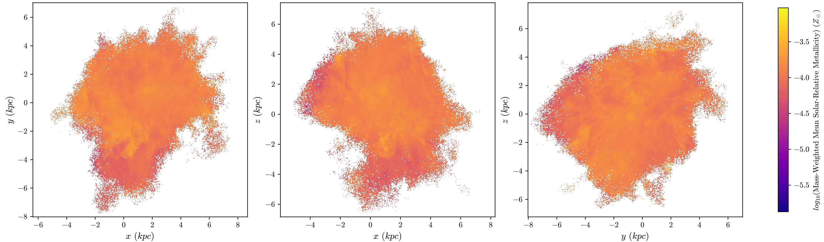
halo8 Mass-Weighted Mean Metallicity, z = 3.491 , 512 bins
