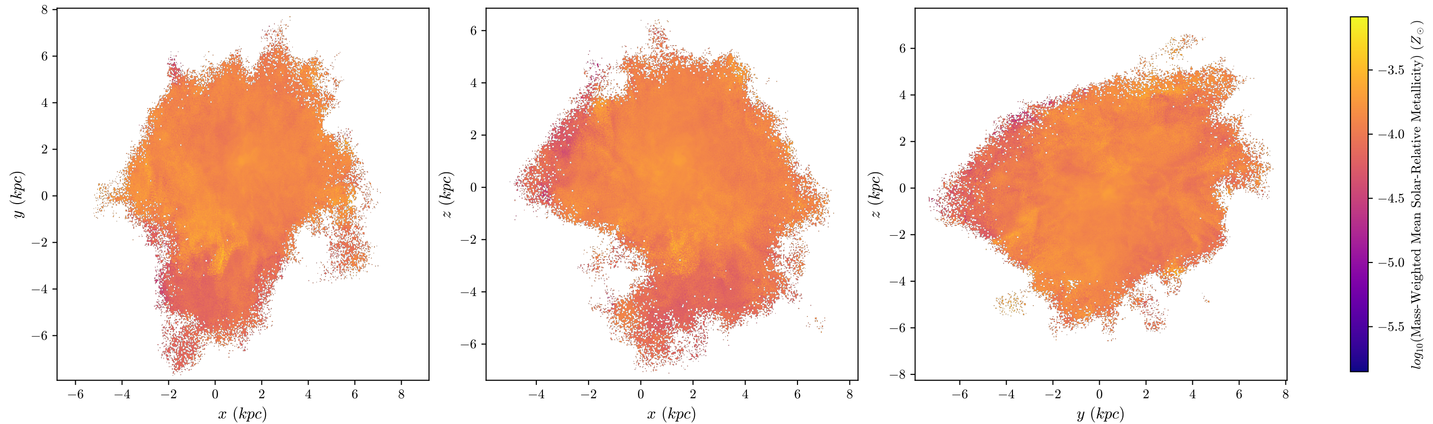
halo8 Mass-Weighted Mean Metallicity, z = 3.47 , 512 bins
