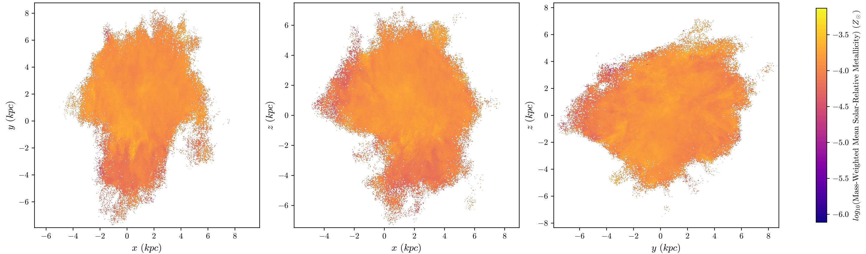
halo8 Mass-Weighted Mean Metallicity, z = 3.427 , 512 bins
