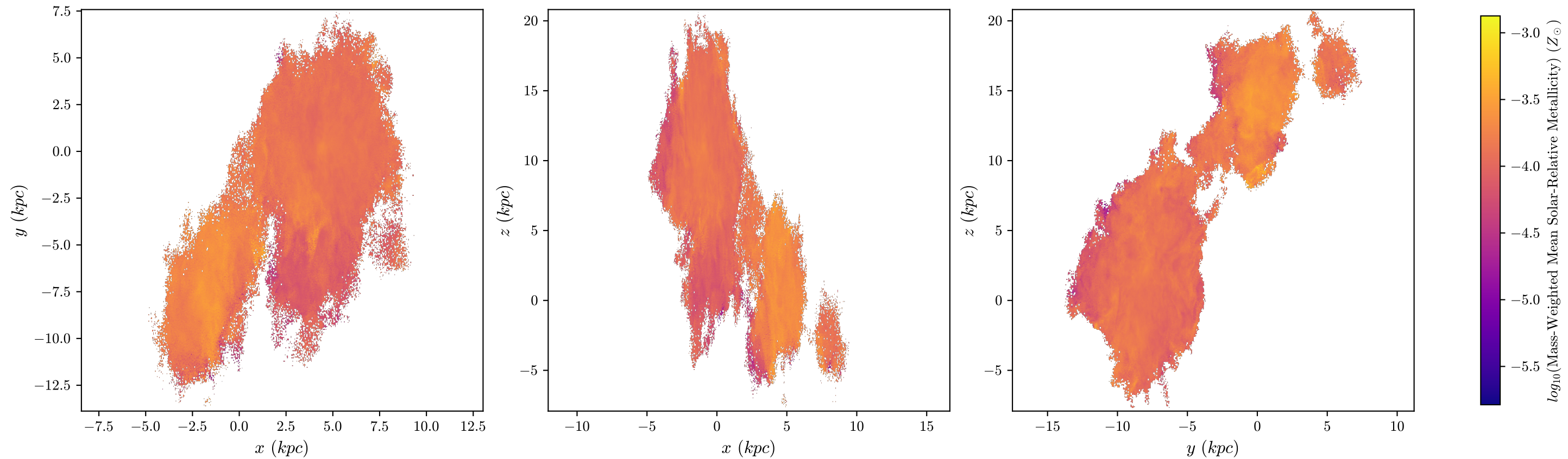
halo8 Mass-Weighted Mean Metallicity, z = 3.386 , 512 bins
