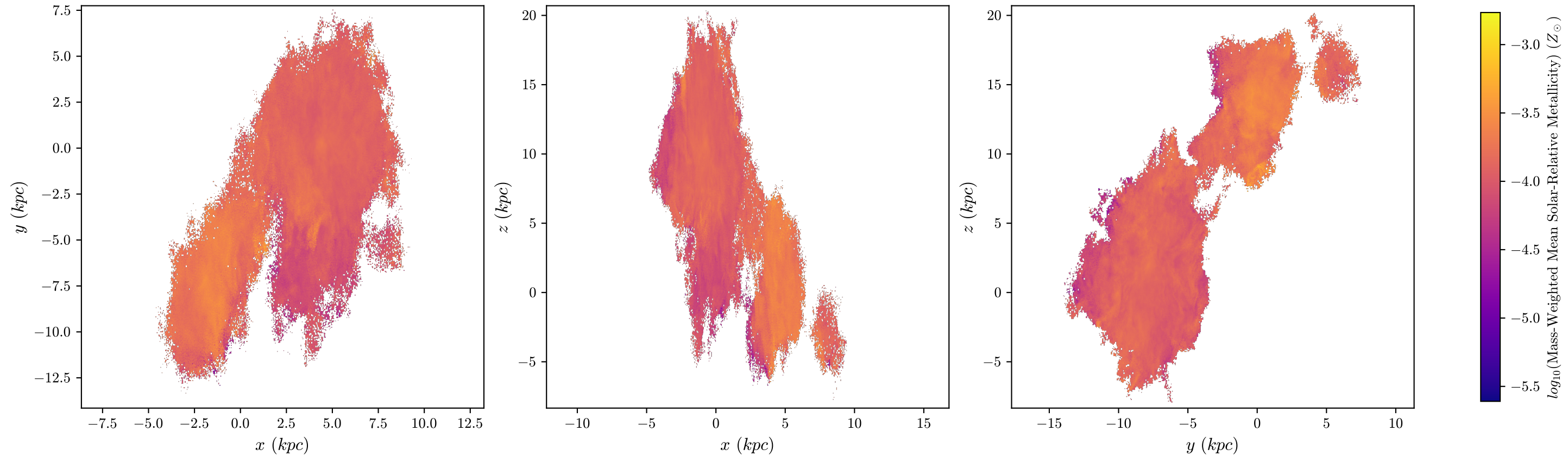
halo8 Mass-Weighted Mean Metallicity, z = 3.365 , 512 bins
