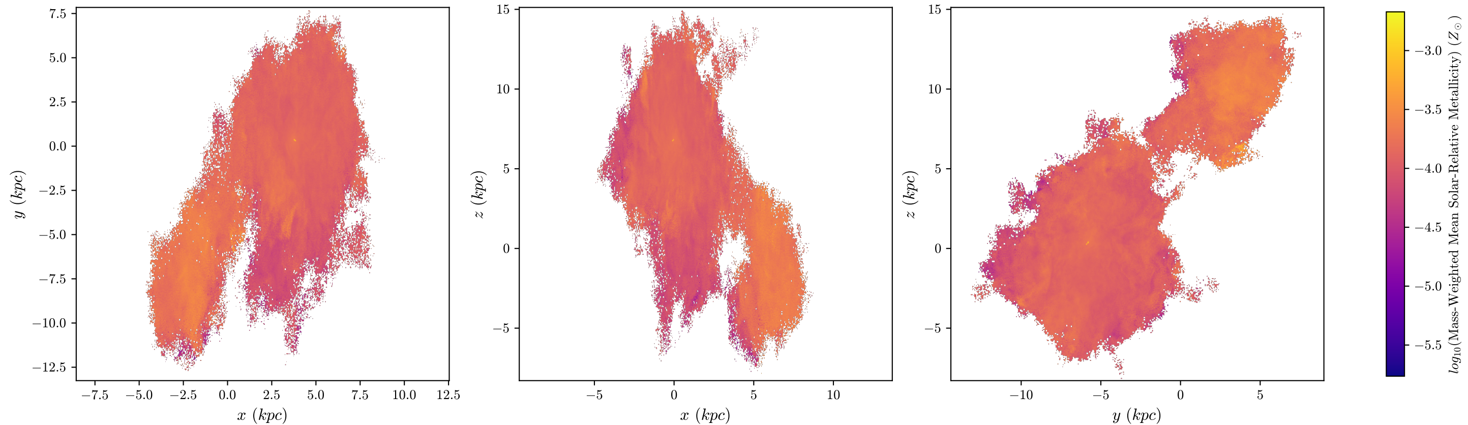
halo8 Mass-Weighted Mean Metallicity, z = 3.324 , 512 bins
