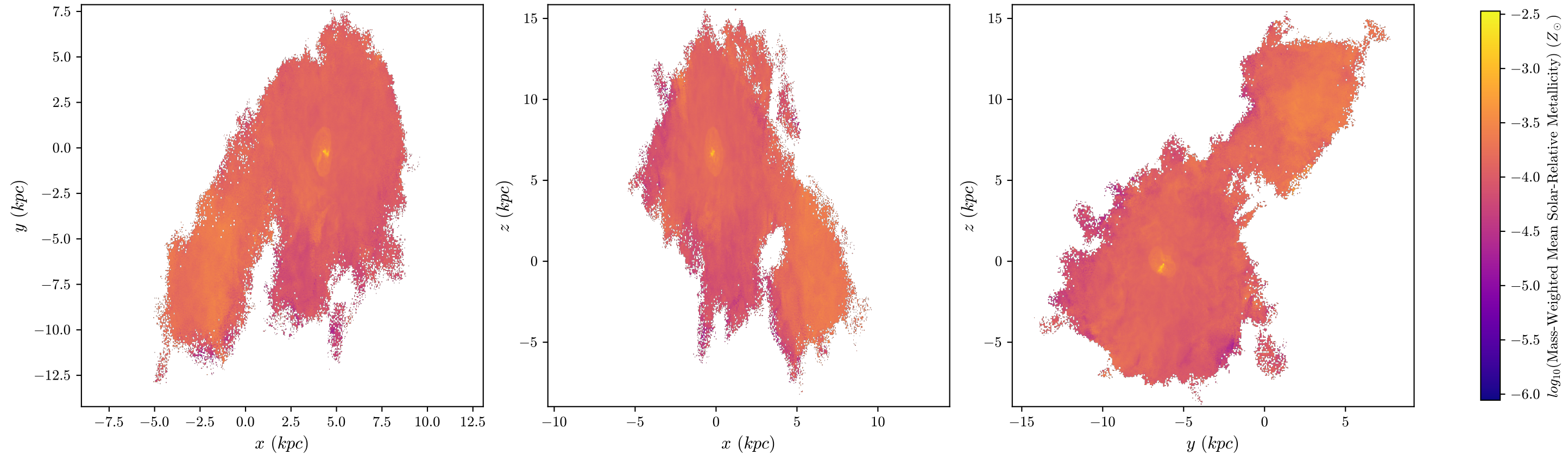
halo8 Mass-Weighted Mean Metallicity, z = 3.263 , 512 bins
