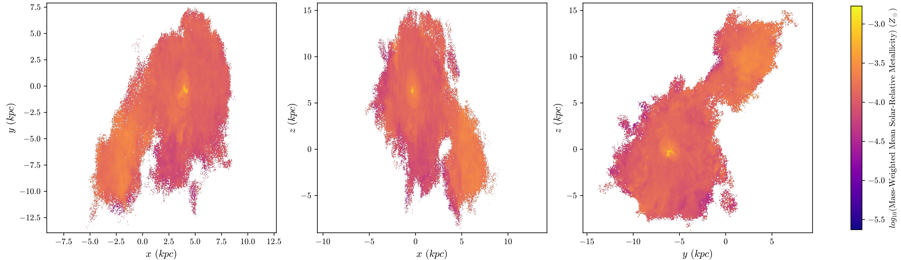
halo8 Mass-Weighted Mean Metallicity, z = 3.243 , 512 bins
