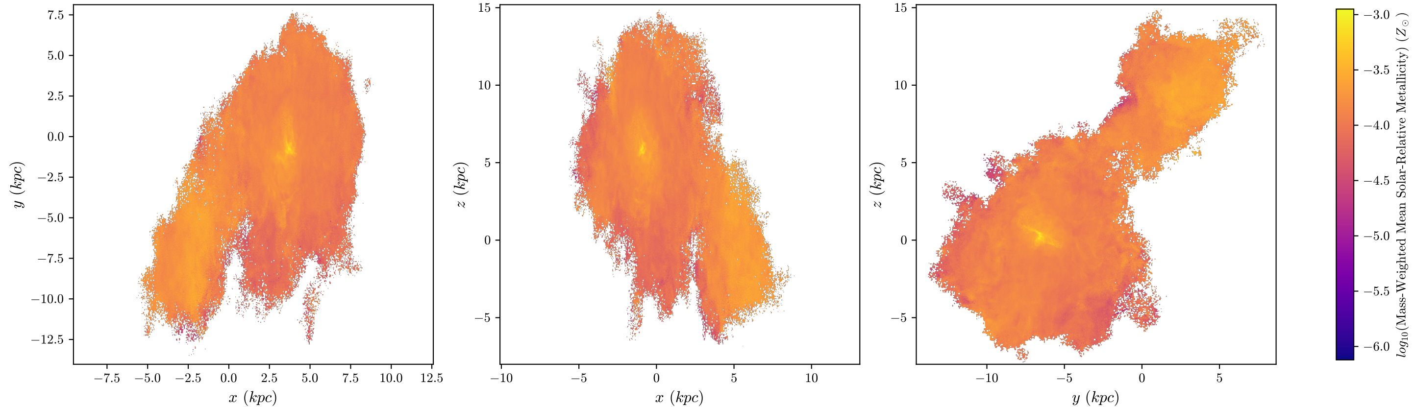
halo8 Mass-Weighted Mean Metallicity, z = 3.203 , 512 bins
