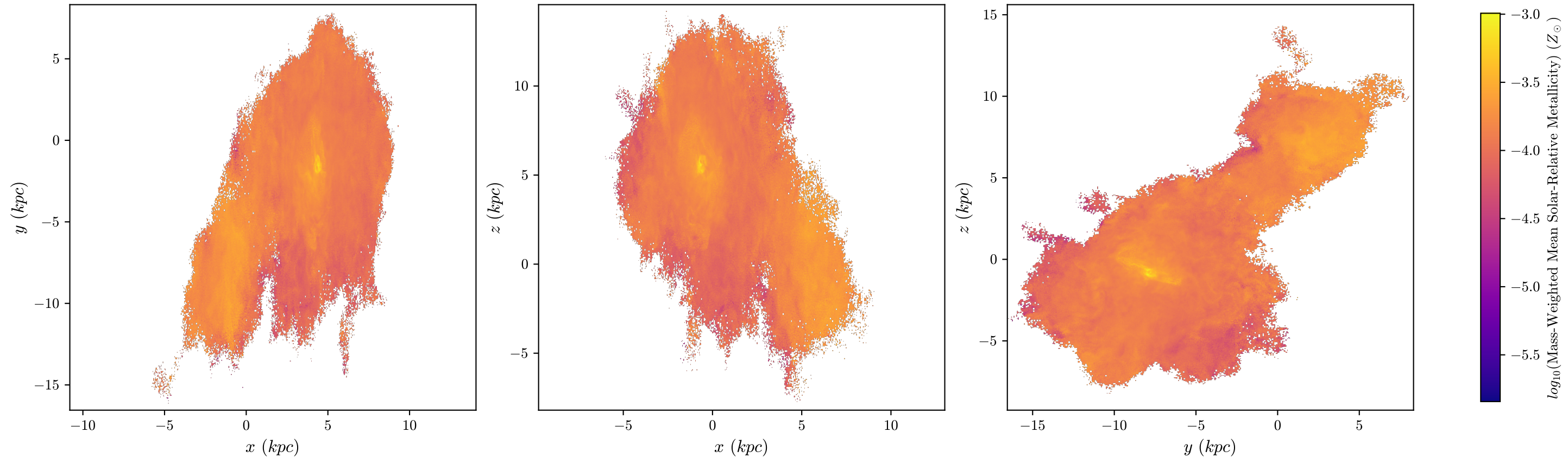
halo8 Mass-Weighted Mean Metallicity, z = 3.163 , 512 bins
