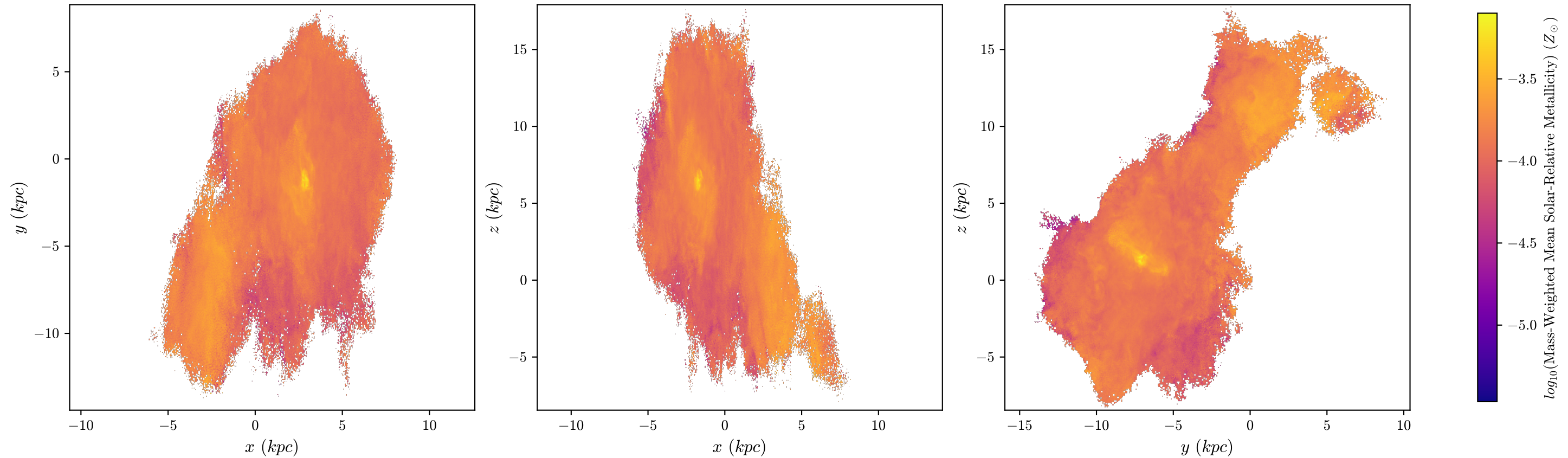
halo8 Mass-Weighted Mean Metallicity, z = 3.104 , 512 bins
