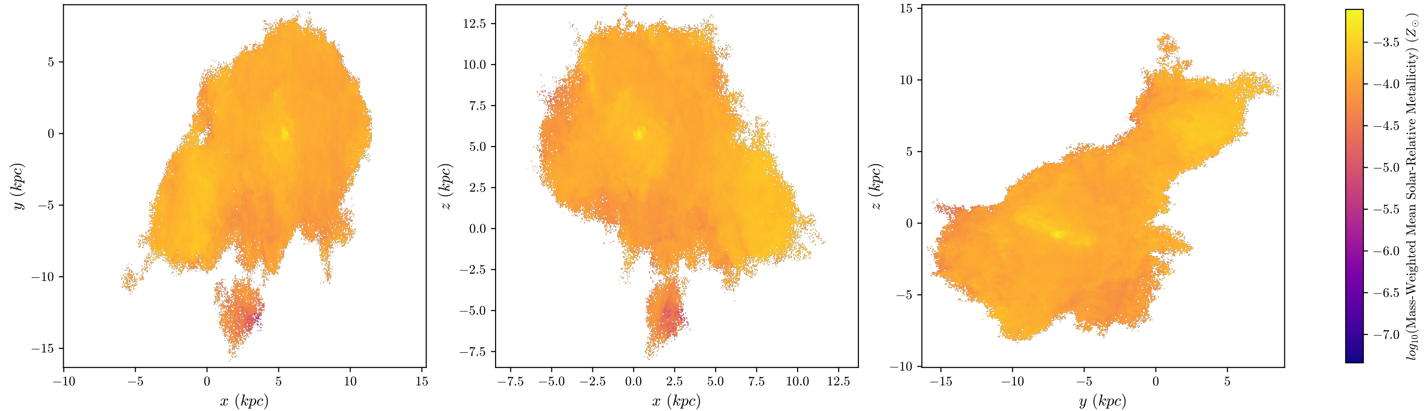
halo8 Mass-Weighted Mean Metallicity, z = 3.085 , 512 bins
