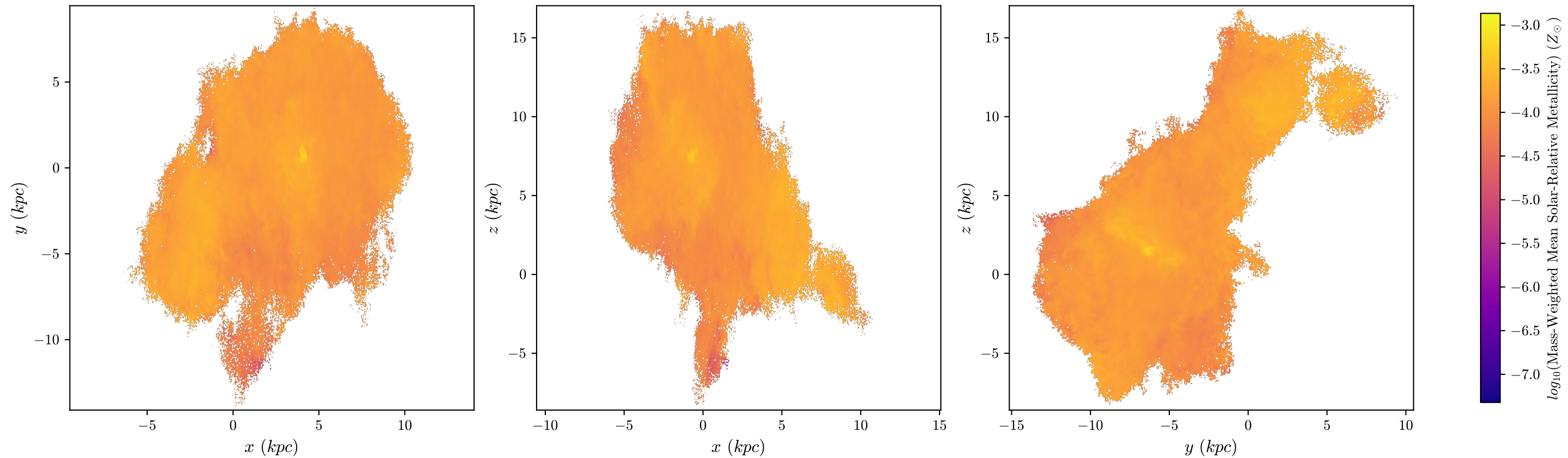
halo8 Mass-Weighted Mean Metallicity, z = 3.046 , 512 bins
