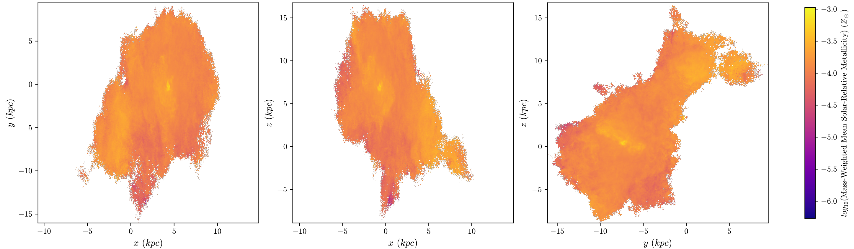
halo8 Mass-Weighted Mean Metallicity, z = 3.027 , 512 bins
