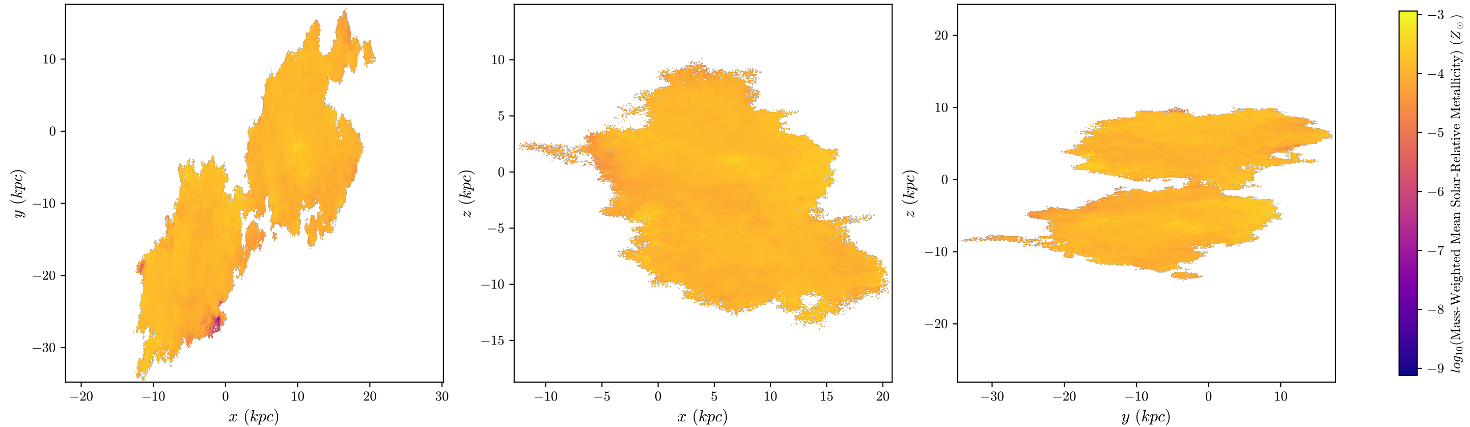
halo8 Mass-Weighted Mean Metallicity, z = 2.544 , 512 bins
