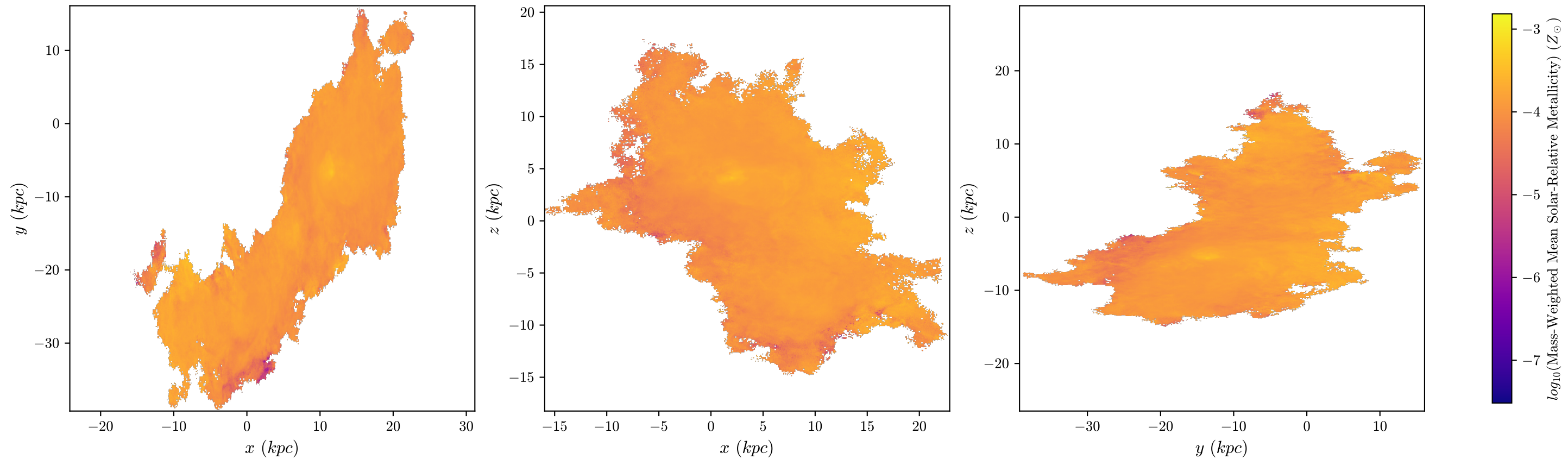
halo8 Mass-Weighted Mean Metallicity, z = 2.178 , 512 bins
