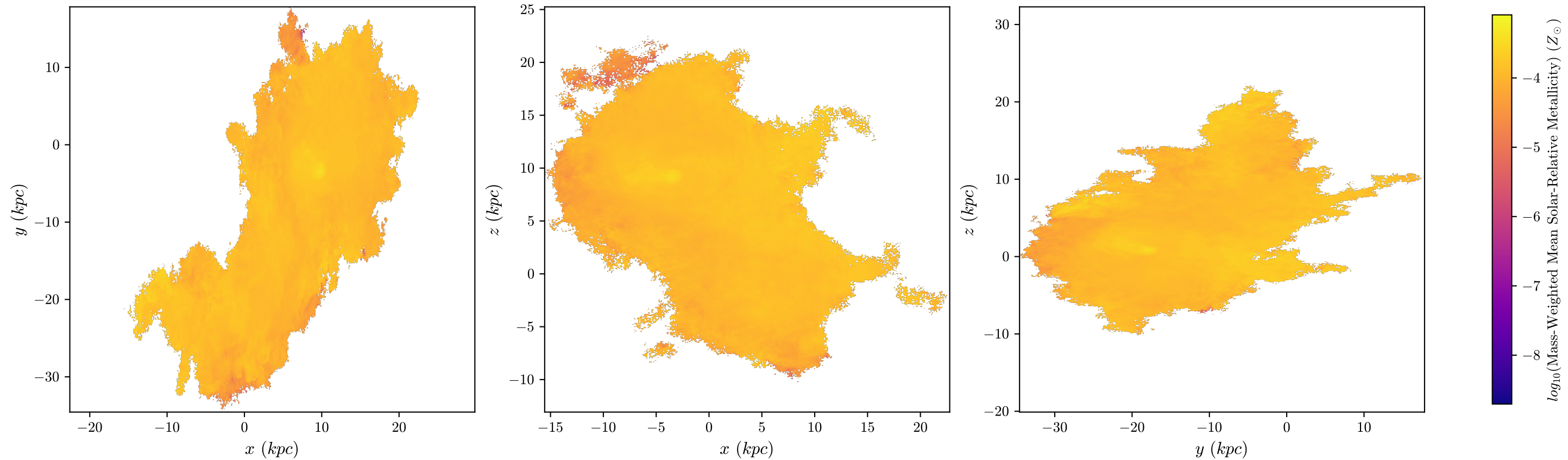
halo8 Mass-Weighted Mean Metallicity, z = 1.904 , 512 bins
