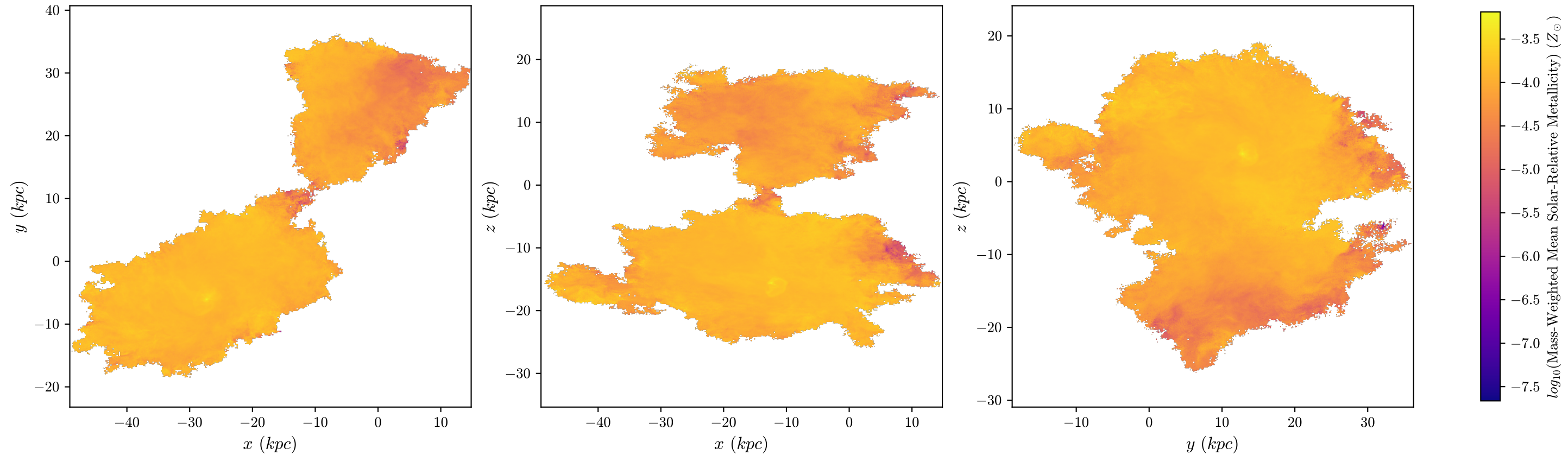
halo8 Mass-Weighted Mean Metallicity, z = 1.496 , 512 bins
