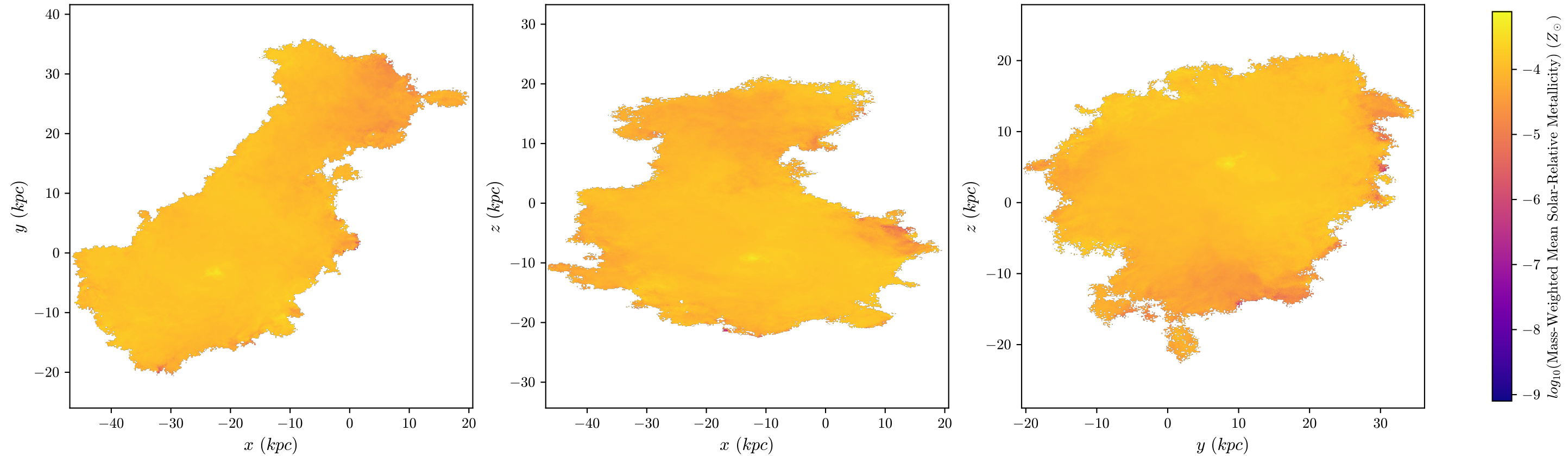
halo8 Mass-Weighted Mean Metallicity, z = 1.324 , 512 bins
