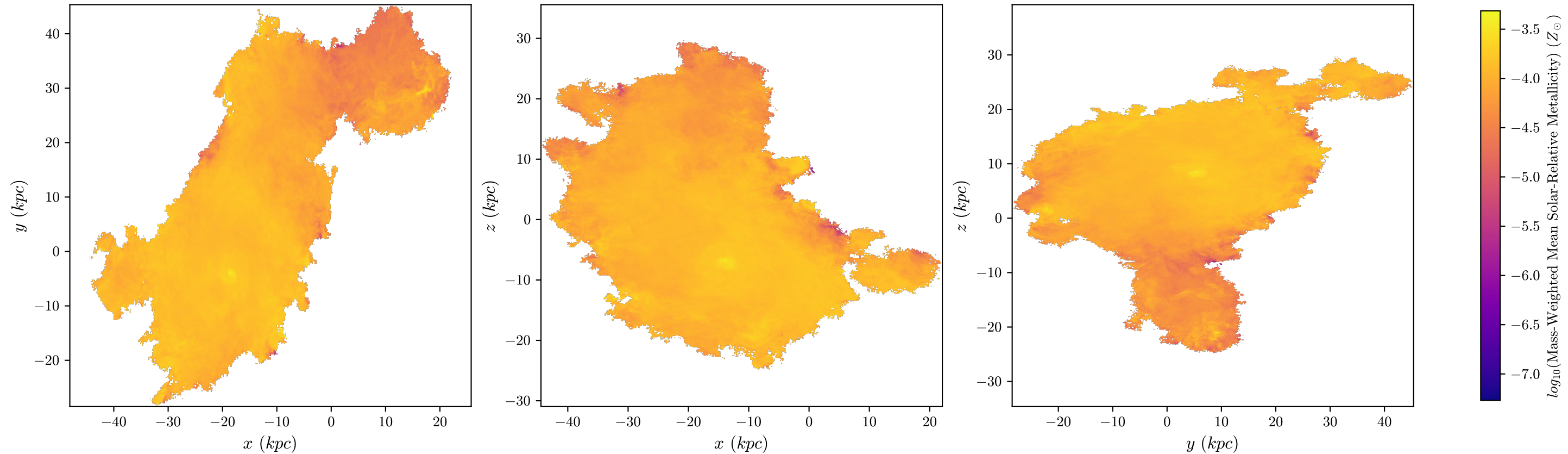
halo8 Mass-Weighted Mean Metallicity, z = 1.185 , 512 bins
