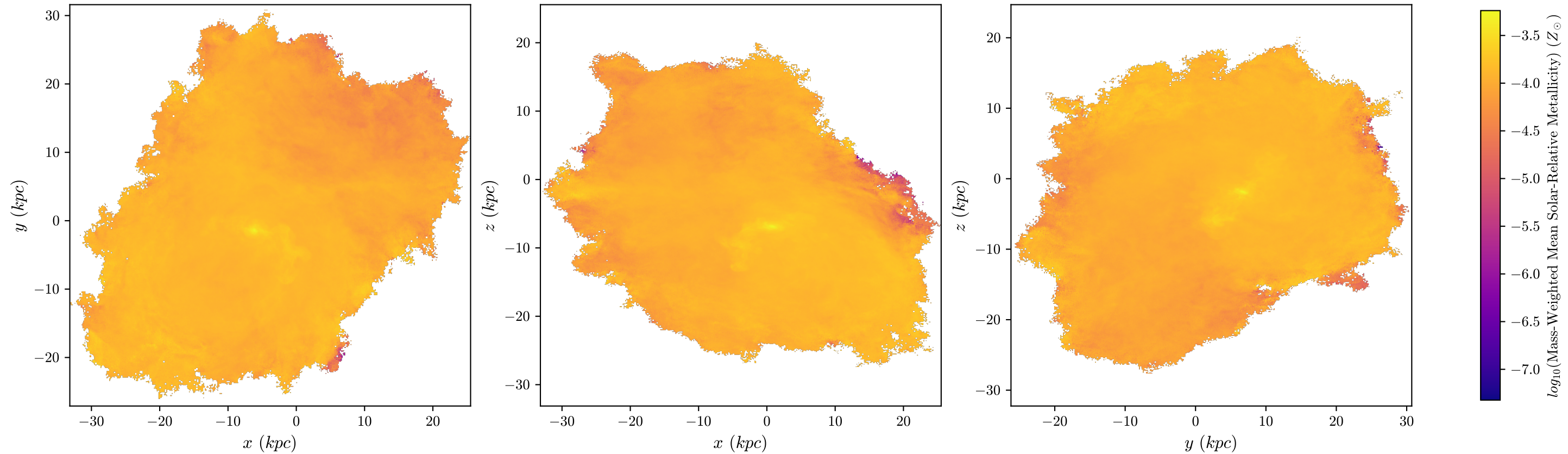
halo8 Mass-Weighted Mean Metallicity, z=0.96 , 512 bins
