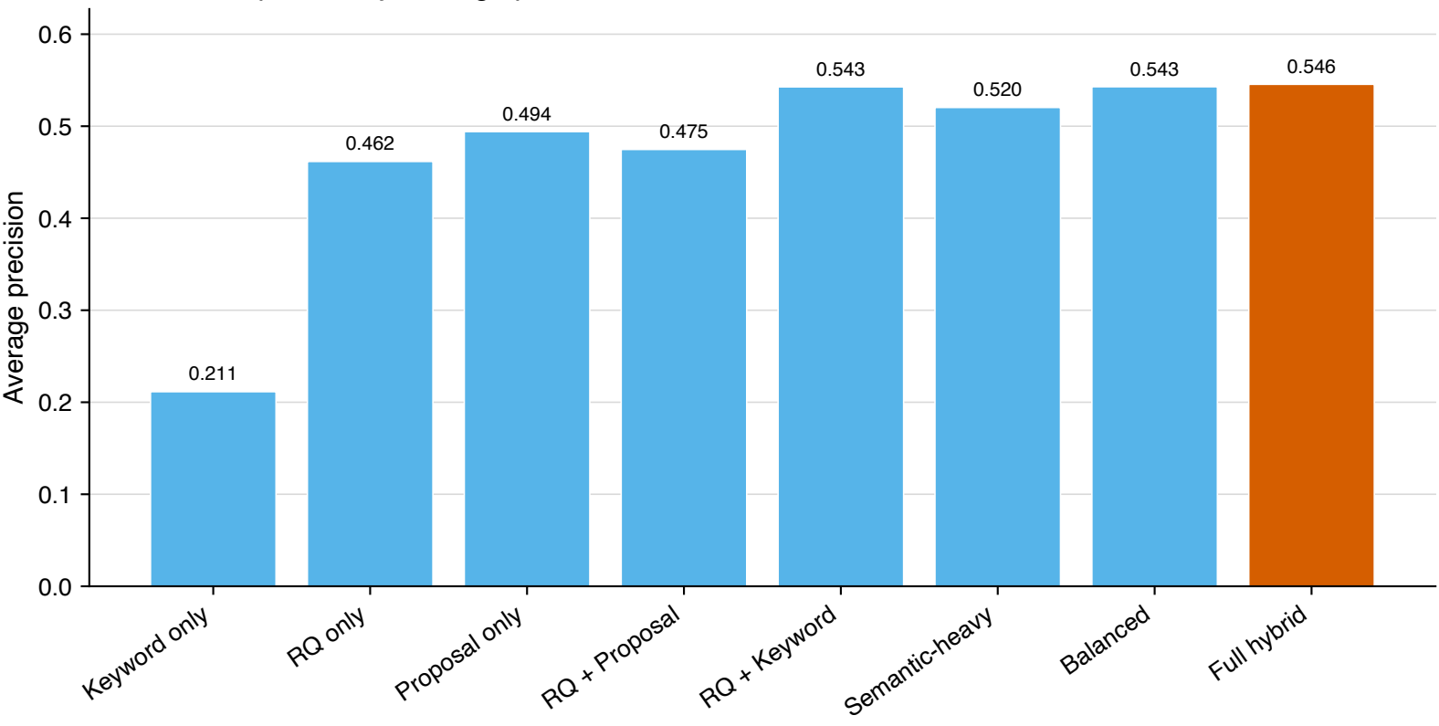
Ablation comparison by average precision
