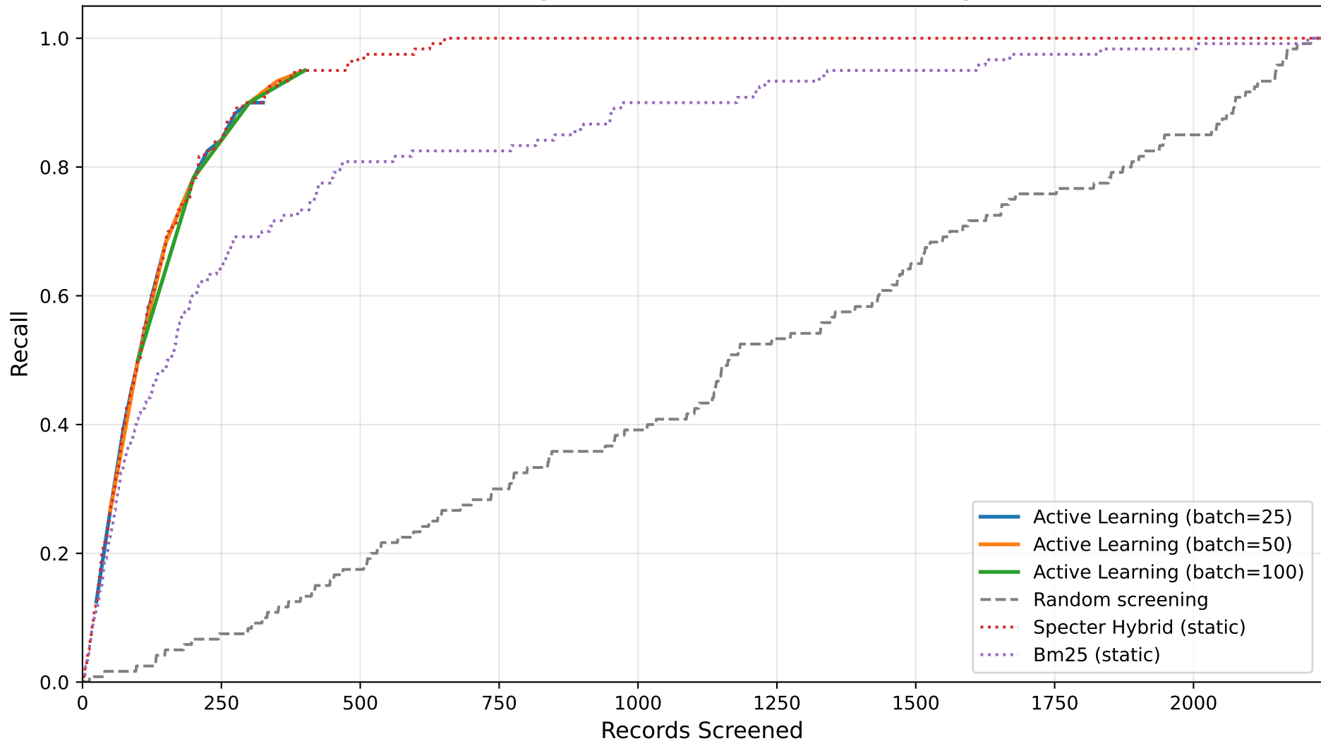
Active Learning Simulation: Recall vs Screening Effort
