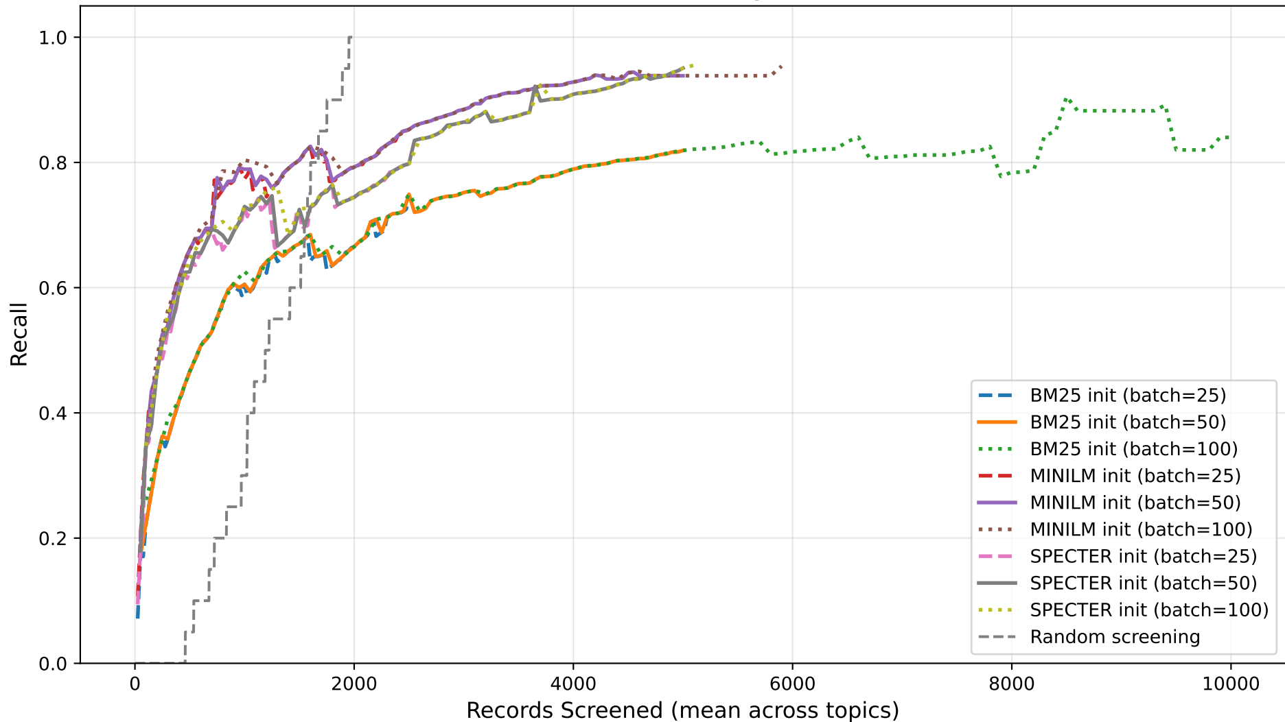
CLEF-TAR: Active Learning Recall Curve
