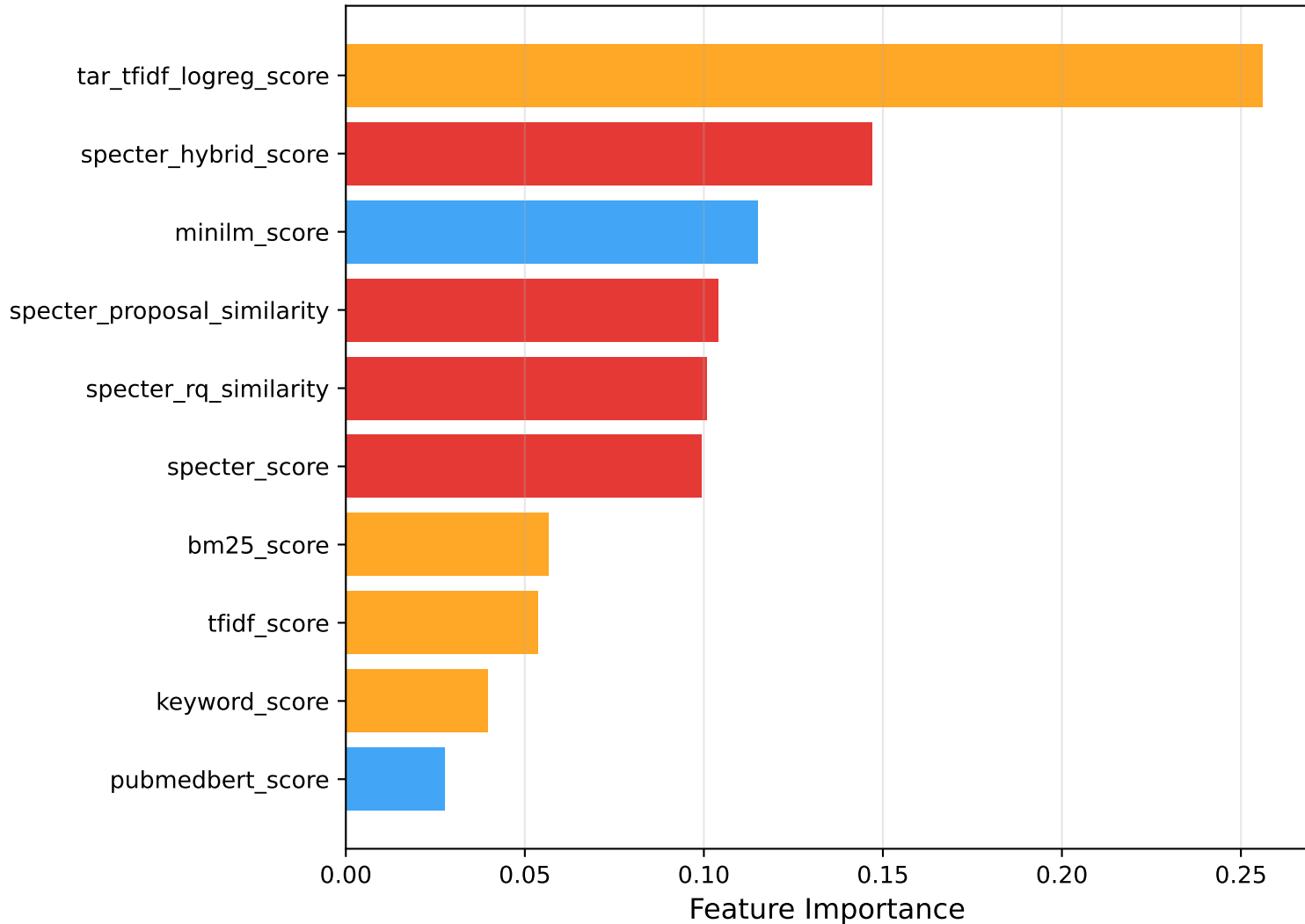
ExtraTrees Feature Importance for Learned Reranker
