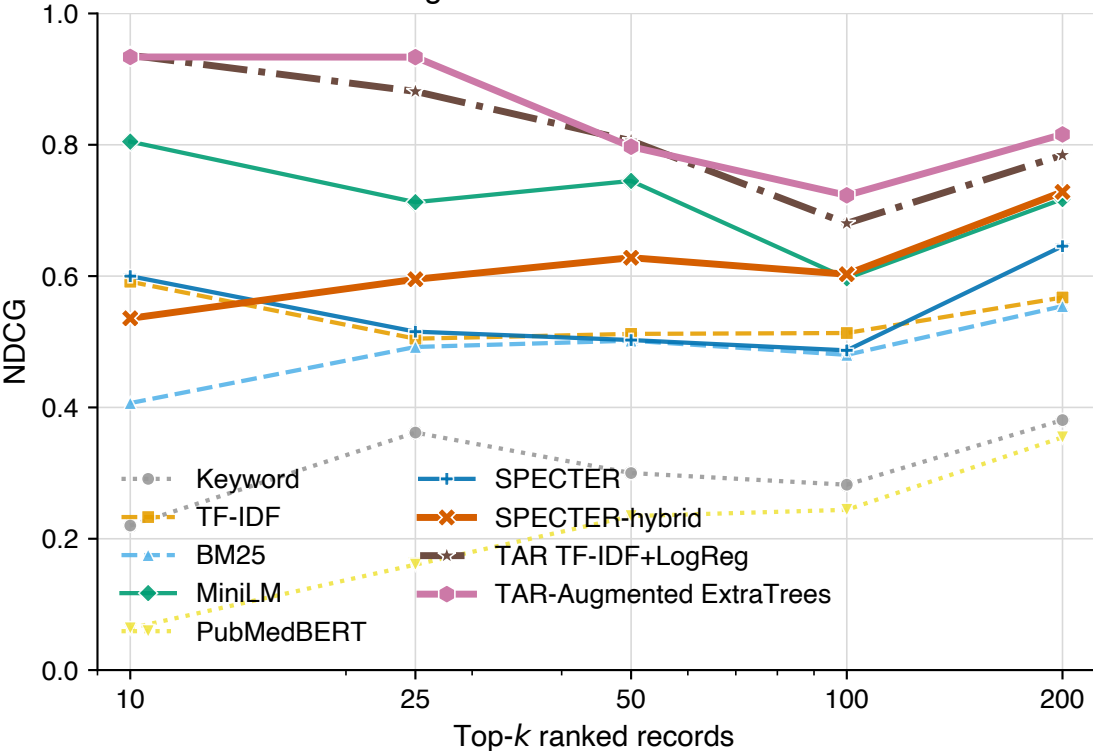
NDCG across screening cut-offs
