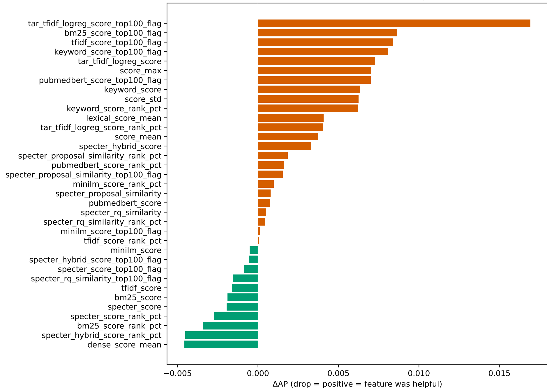
Leave-One-Feature-Out Ablation: Average Precision
