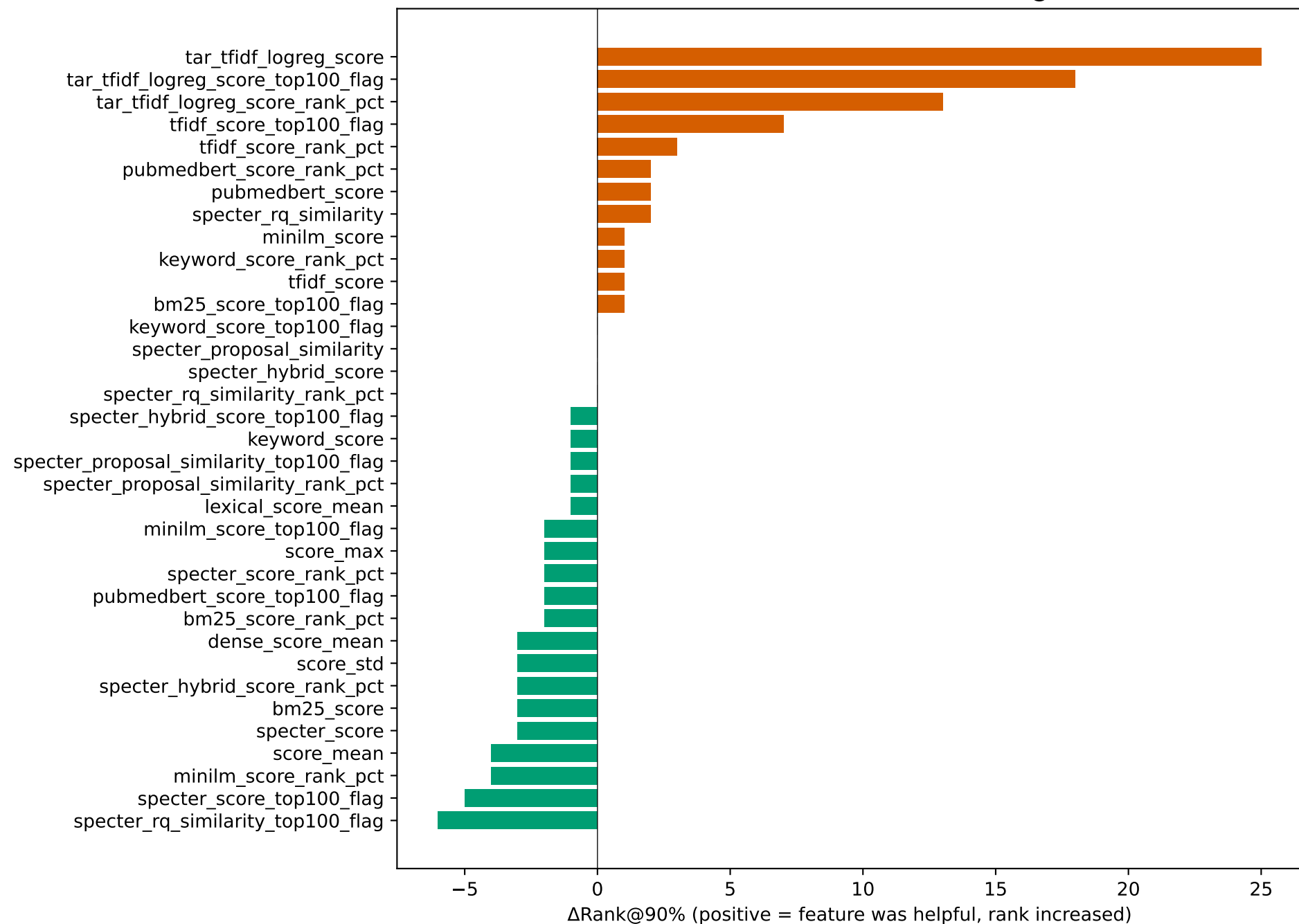
Leave-One-Feature-Out Ablation: Rank@90%
