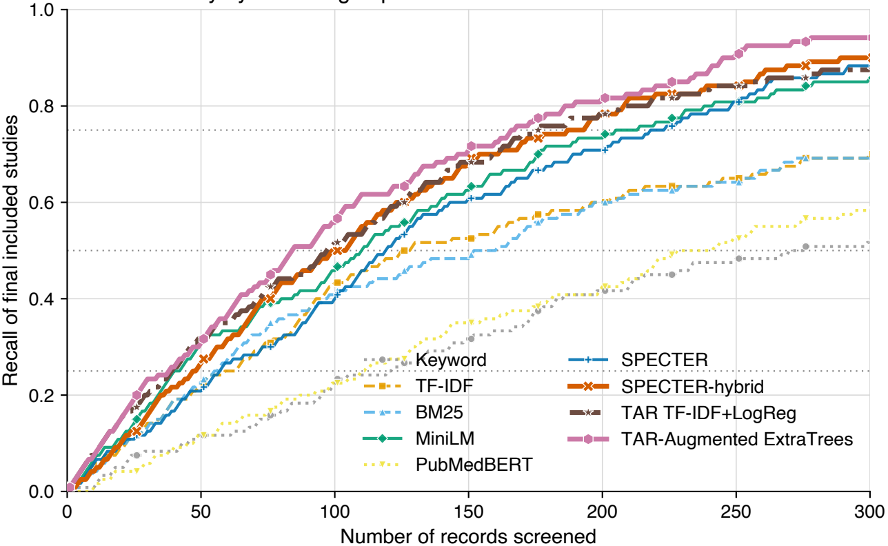
Recall recovery by screening depth
