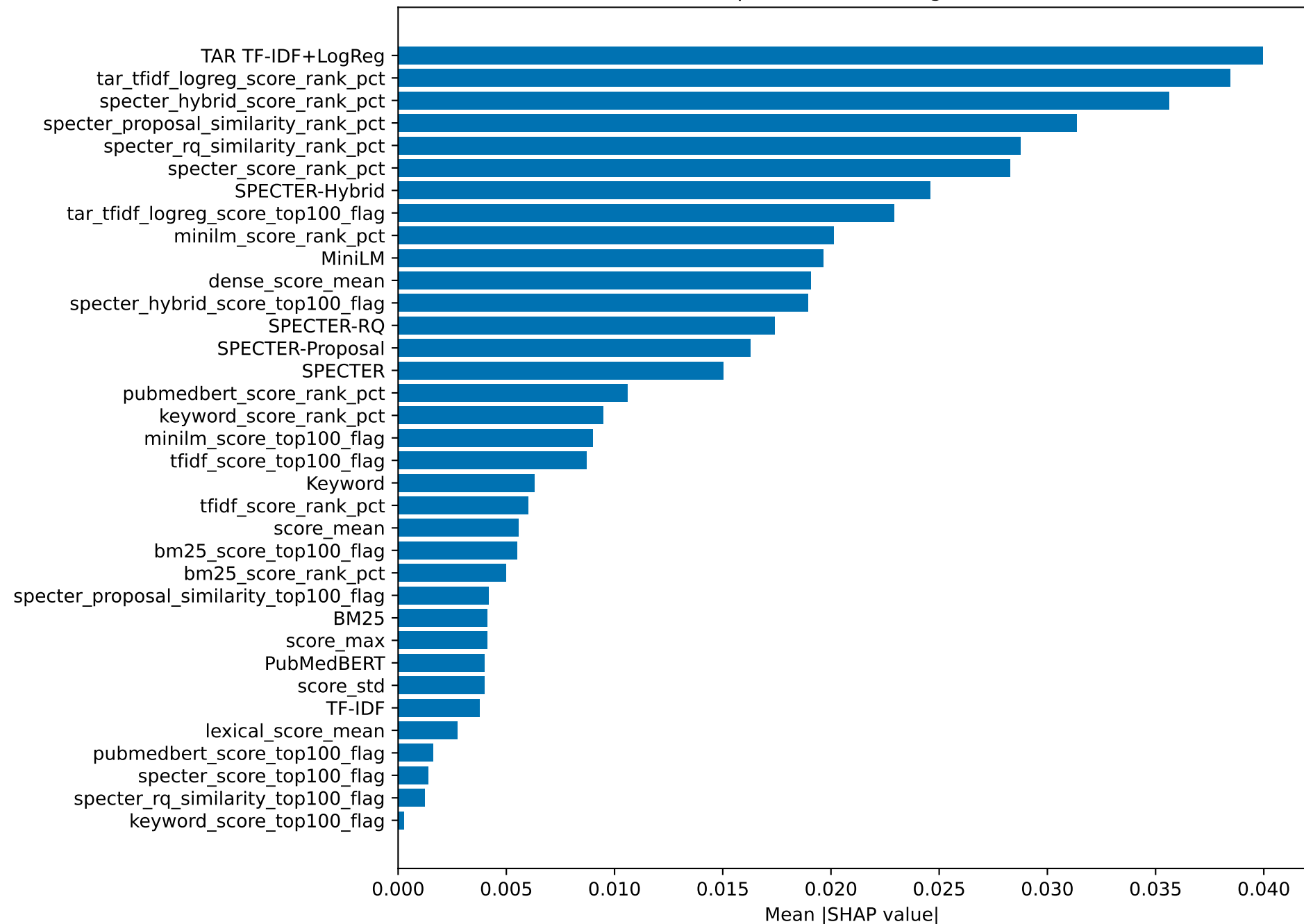
SHAP Feature Importance: TAR-Augmented ExtraTrees
